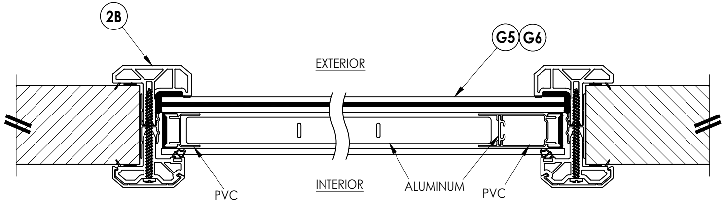
2/4 HORIZONTAL CROSS SECTION WARMEDGE OPERABLE BLIND NOTE: FIXED BLIND NOT SHOWN
